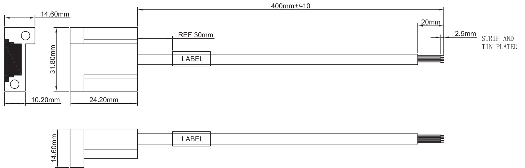
HALL EFFECT WIRING DIAGRAM
