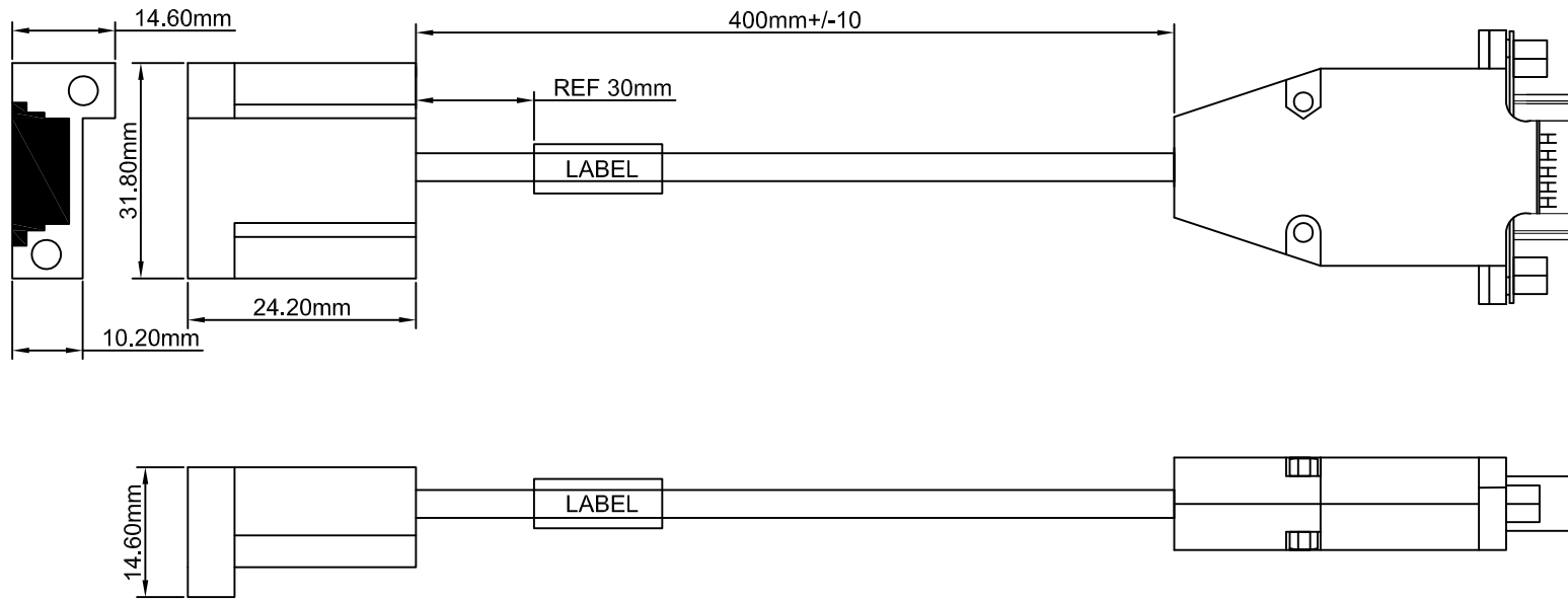
HALL EFFECT WIRING DIAGRAM
