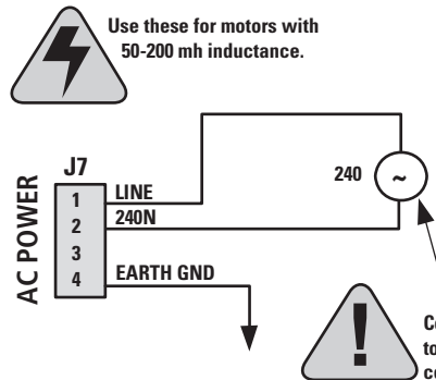
Figure 1a: Connection for a 320 VDC bus using 240 VAC.
