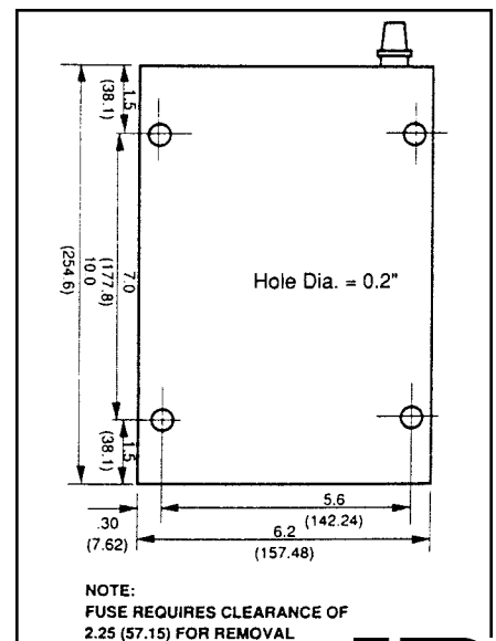
Mounting Diagram
