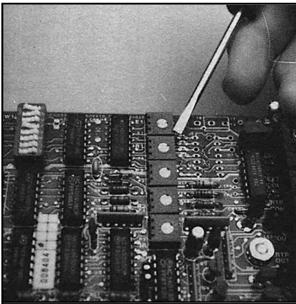
Potentiometer E1 adjusts extension speed, potentiometer R1 adjusts retraction speed
