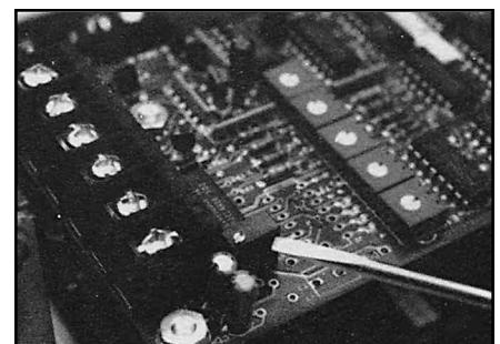
Potentiometer P7 adjusts the length of time delay in example #4.
